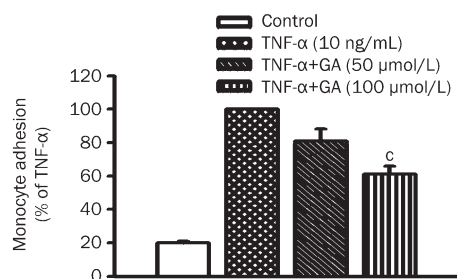
Figure 3. GA inhibits monocyte adhesion to TNF- \alpha -activated HUVEC. Cells pretreated with GA (50 or 100 \mu mol/L) for 3 h were coincubated with TNF- \alpha (10 ng/mL) for another 8 h. [ 3 H]thymidine-labeled monocytic THP-1 cells were added and incubated for 30 min after TNF- \alpha incubation. HUVEC were lysed after removal of nonadherent THP-1 cells, and total radioactivity of cell lysate was counted by liquid scintillation. Data represent mean \pm SEM obtained from 5 independent experiments. c P <0.01 vs TNF- \alpha treatment only.
